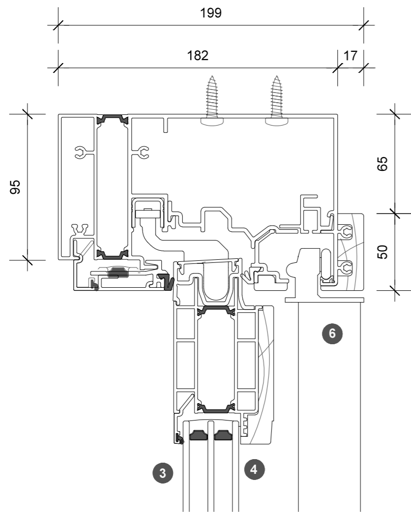
4. head detail
